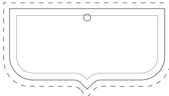
Heijastin 66 x 34mm Aineisto 71 x 39mm Helsinki kehystunnus Reflector 66 x 34mm Artwork 71 x 39mm Used also for the city of Helsinki
